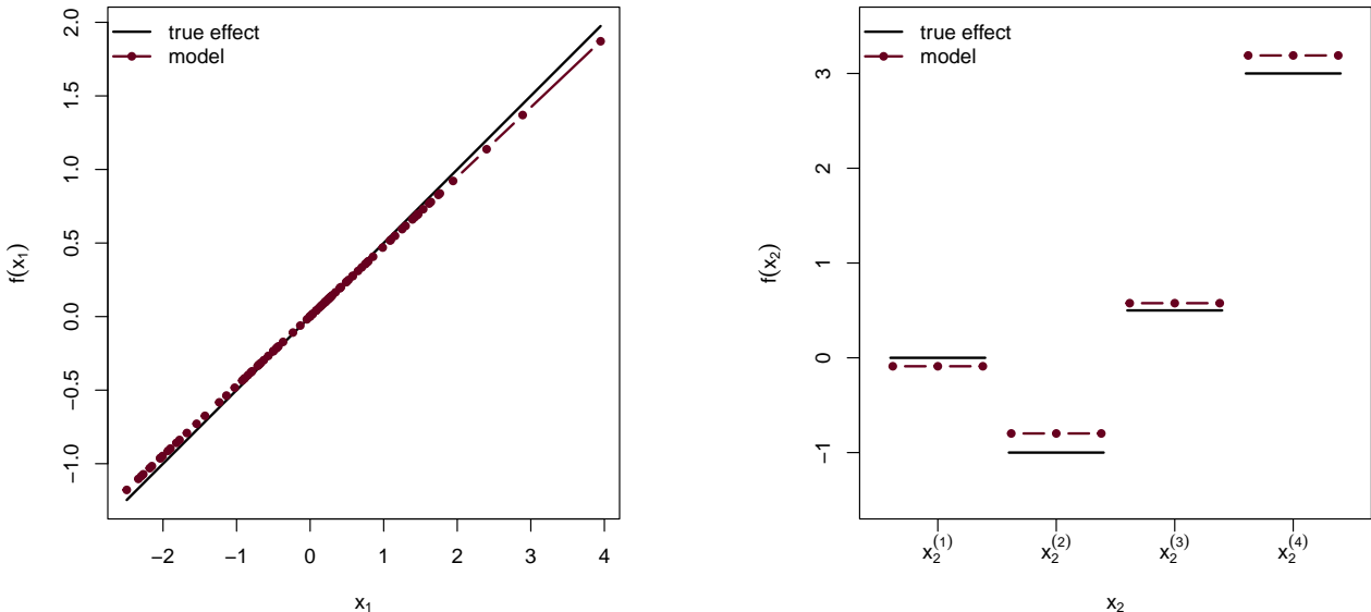
Figure 3: Examples for linear and categorical effects estimated using bo1s() : Linear effect (left; f(x_1) = 0.5x_1 ) and categorical effect (right; f(x_2) = 0x_2^{(1)} - 1x_2^{(2)} + 0.5x_2^{(3)} + 3x_2^{(4)} ). The effects can be estimated with base-learners bo1s(x1) and bo1s(x2) , where x1 is a continuous covariate and x2 is a categorical covariate coded as factor in R.
